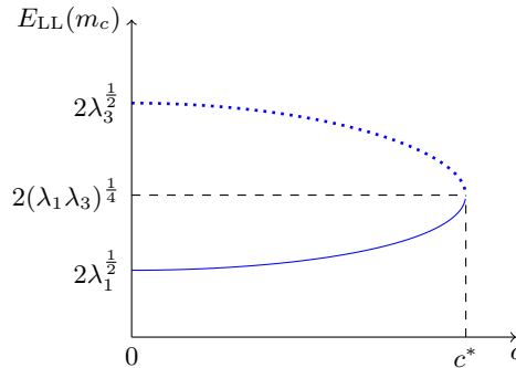
Figure 1: The curves E_{\text{LL}}(m_c^+) and E_{\text{LL}}(m_c^-) in dotted and solid lines, respectively.
